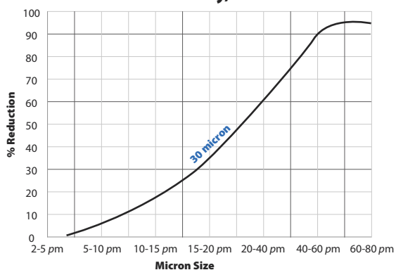
Filtration Efficiency, Pleated
