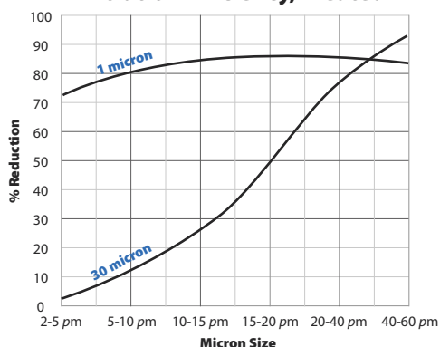
Filtration Efficiency, Pleated
